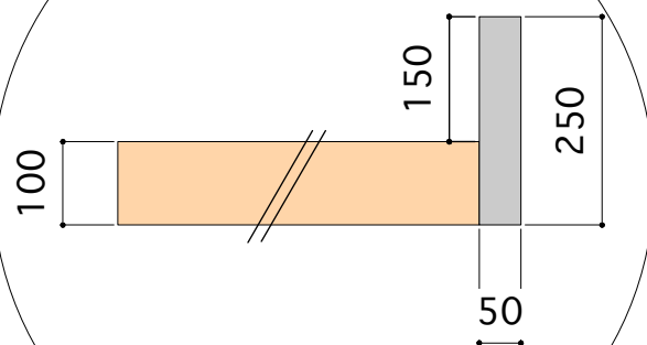
Installation drawing of outer peripheral fence.
